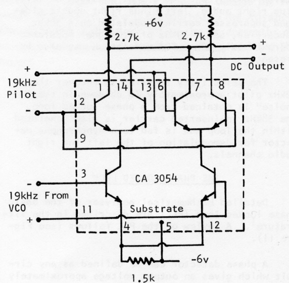
Fig. 4 The Phase Detector
