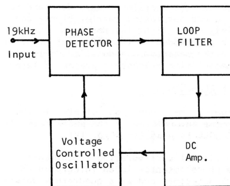
Fig. 2 Basic Phase Locked Loop
