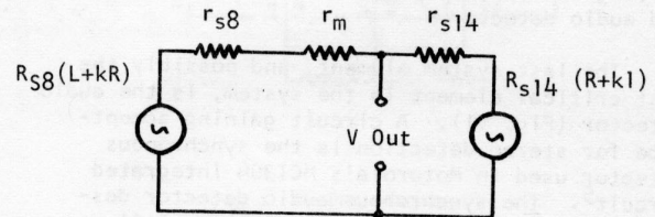
Fig. 9 Resulting Equivalent Circuit
