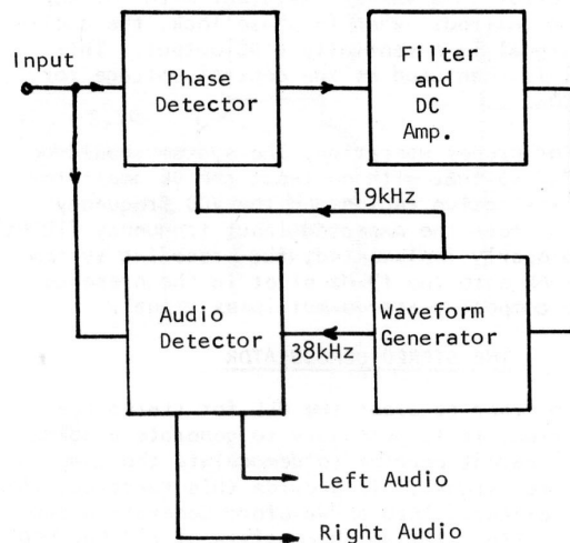
Fig. 1 Stereo Multiplex Demodulator
